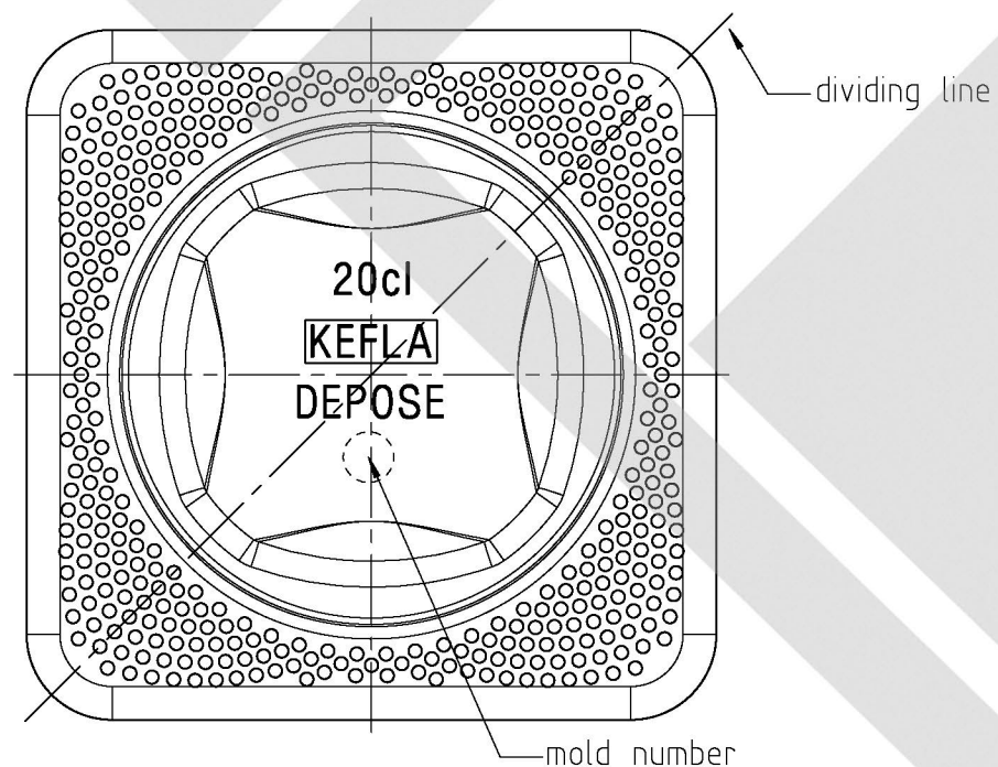
BOTTOM VIEW
